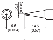
T18-DL12 SHAPE-1.2DL
